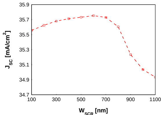
Figure 6. J_{sc} as a function of SCR width.
