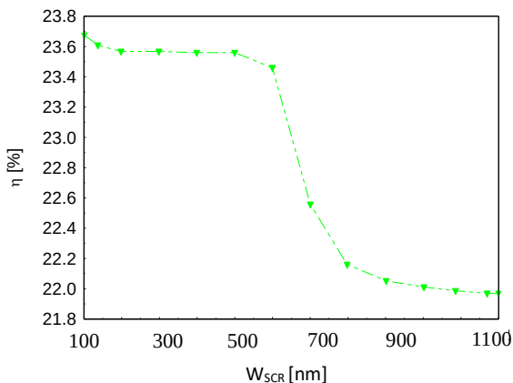
Figure 7. Conversion efficiency as a function of SCR width.
