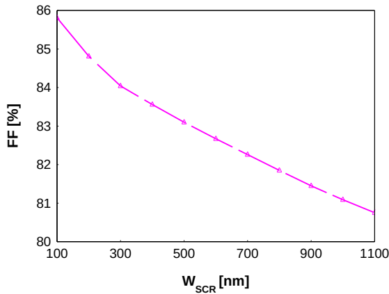
Figure 5. FF as a function of SCR width.
